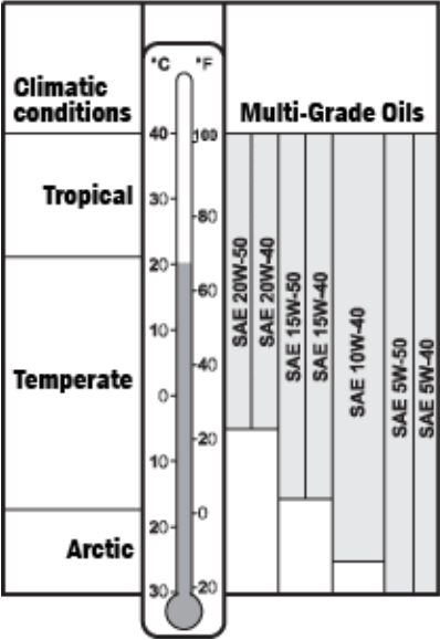
FIGURE 8-1 VISCOSITY
