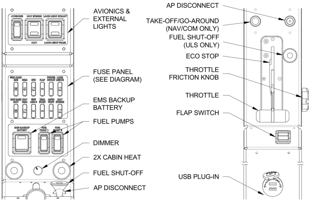
FIGURE 7-5 RV-12iS CONSOLE, FUEL SHUT-OFF INSTALLED
