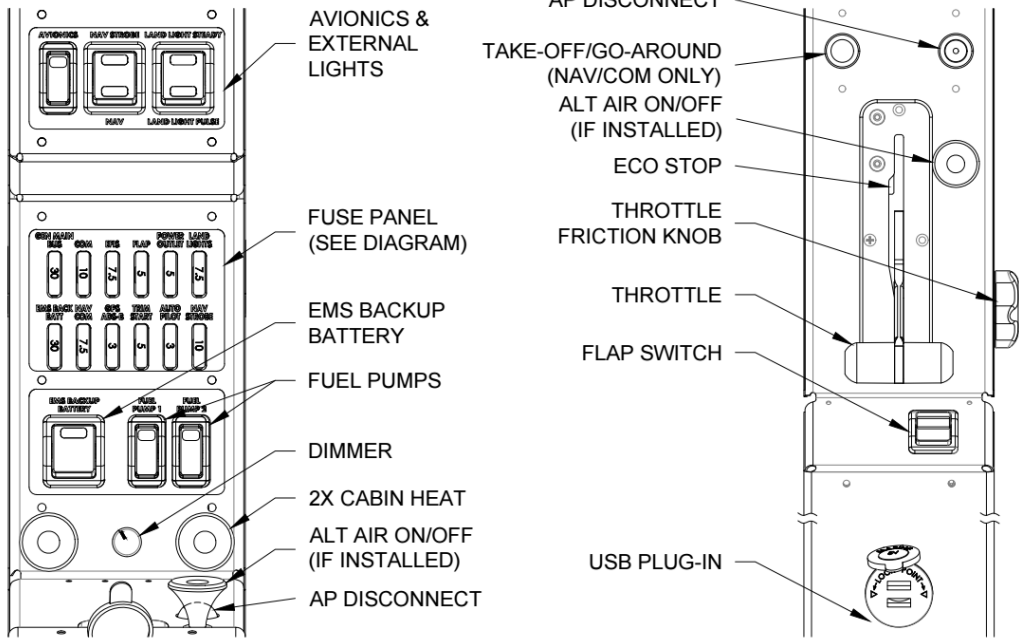
FIGURE 7-5 RV-12iS CONSOLE, FUEL SHUT-OFF INSTALLED
