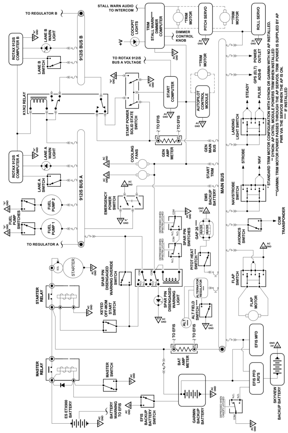
FIGURE 7-8 ROTAX 912 IS ELECTRICAL SYSTEM
