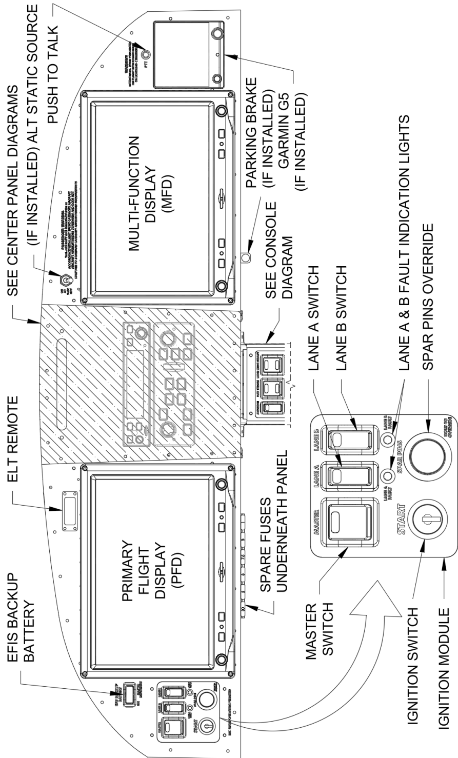
FIGURE 7-3 RV-12iS INSTRUMENT PANEL RV-12iS PILOT'S OPERATING HANDBOOK
