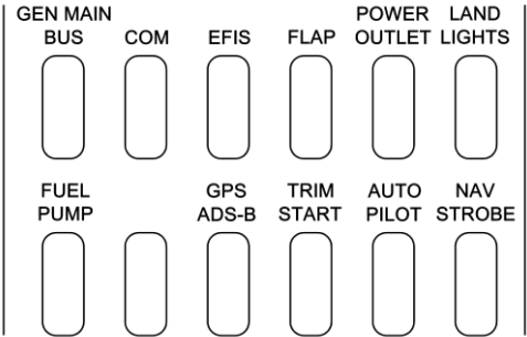
FIGURE 7-11 FUSE PANEL DIAGRAM - ULS
