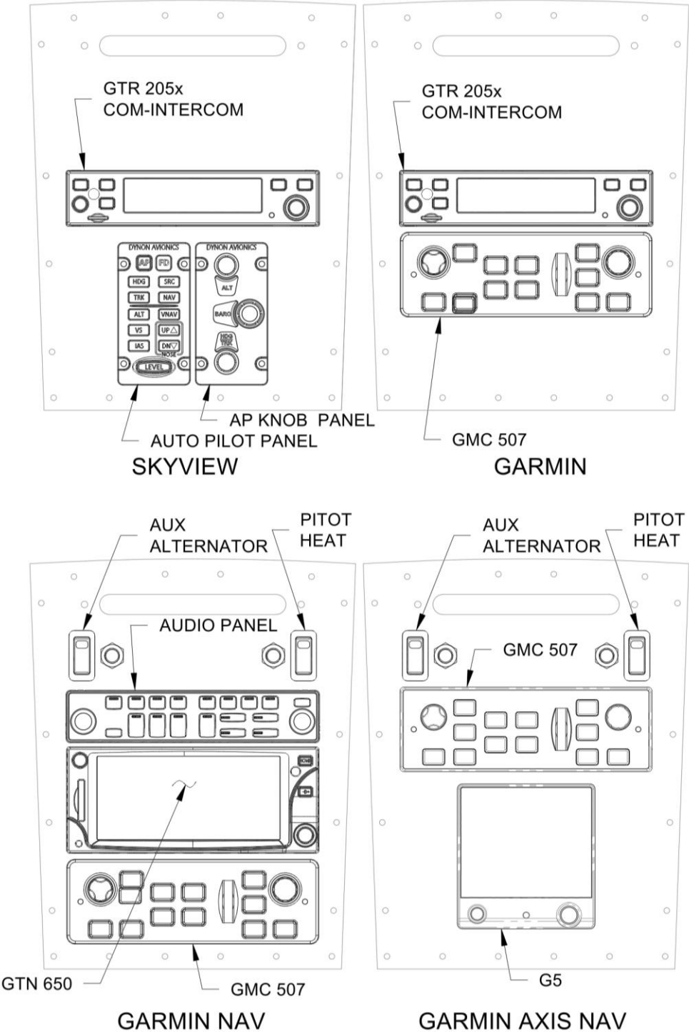
FIGURE 7-4 CENTER PANEL CONFIGURATIONS
