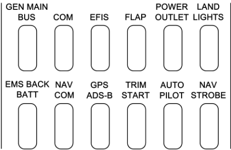
FIGURE 7-10 FUSE PANEL DIAGRAM - iS
