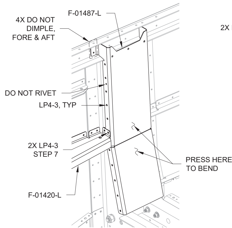
FIGURE 1: CENTER SECTION CHANNEL
