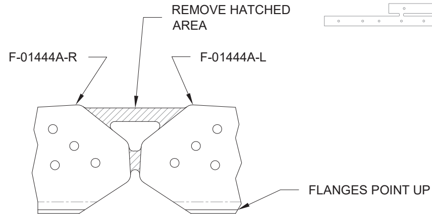
FIGURE 2: SEPARATE LONGERON DOUBLER
