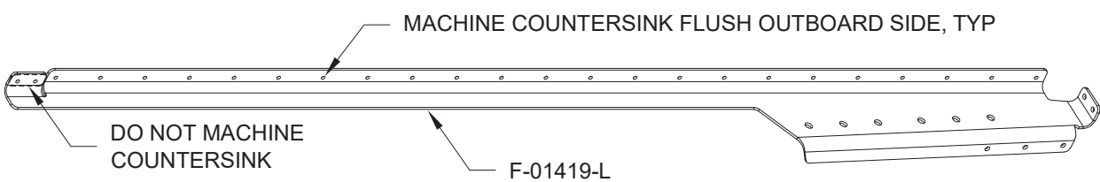
FIGURE 2: MACHINE COUNTERSINKING
