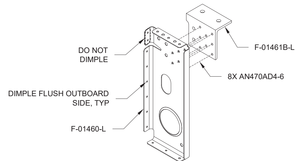
FIGURE 3: INTERCOSTAL
