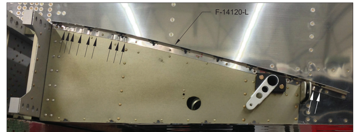
FIGURE 3: SUGGESTED F-14120-L WING ROOT FAIRING FLUTING
