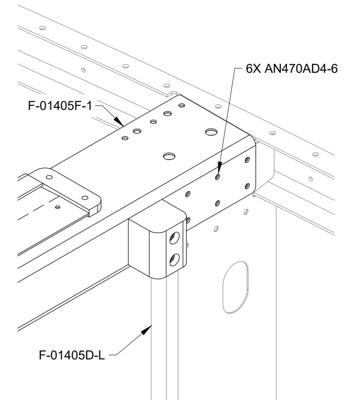
FIGURE 3: BRACE INSTALLATION
