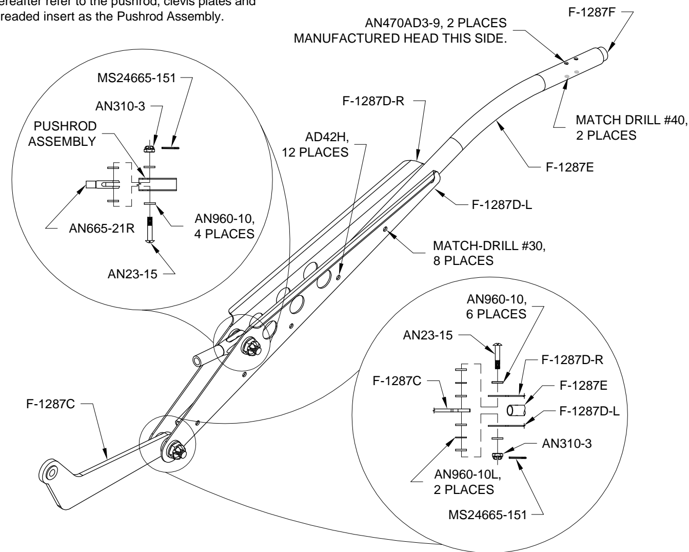
FIGURE 1: PUSHROD ASSEMBLY
