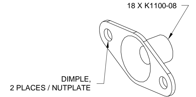
FIGURE 3: NUTPLATE PREPARATION
